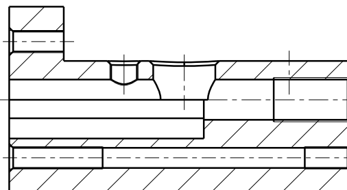
截面/Section A-A
