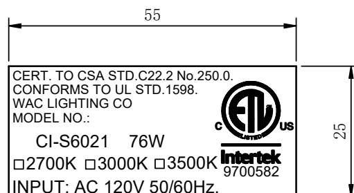
FOR CI-MT-S6012-KIT
