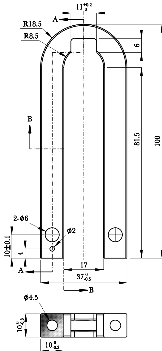
铝挤截面 B-B Aluminium extrusion cross section
