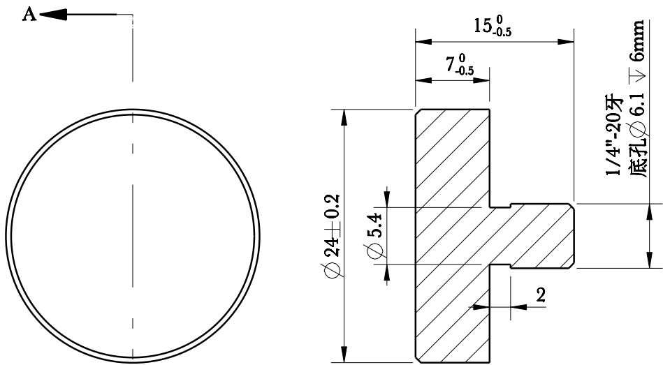
截面/Section A-A
