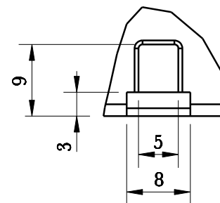
细节/View Details A 比例/Scale 3:2
