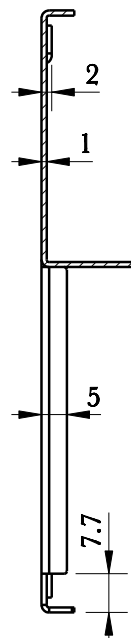
截面/Section A-A
