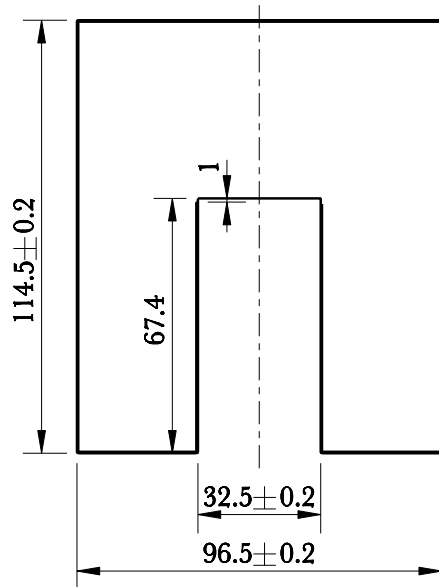
截面/Section A-A
