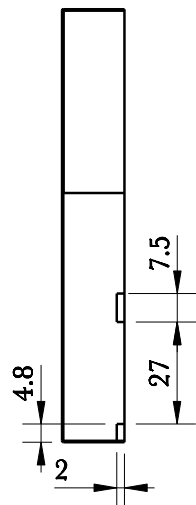
截面/Section A-A
