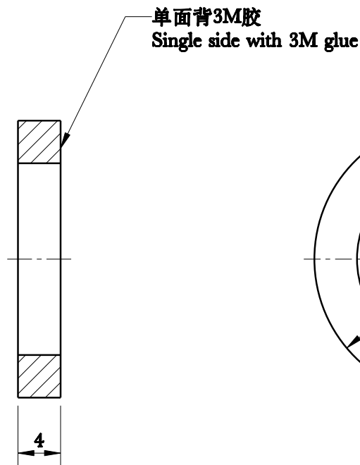
截面Sectin A-A
